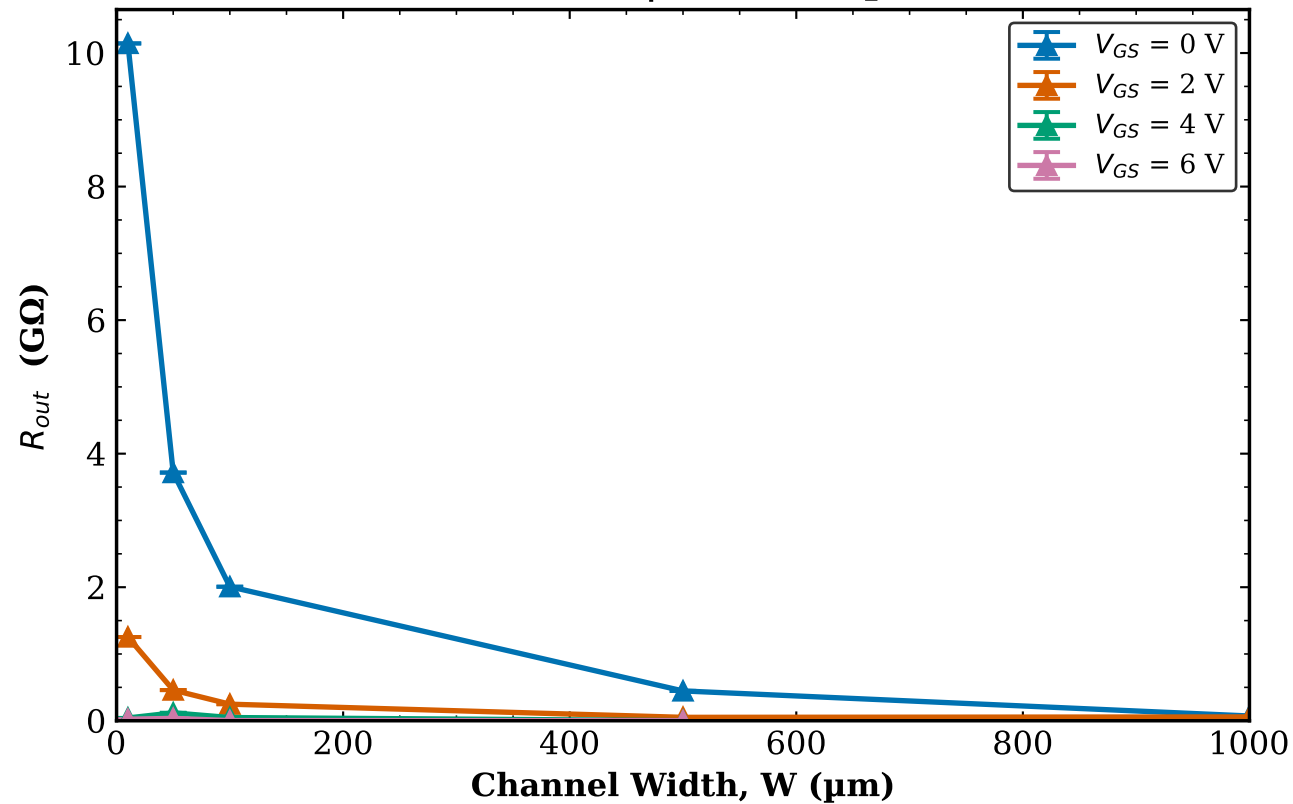
TFT2 Transistor 2 R_{out} vs W | L = 160\text{ }\mu\text{m}
